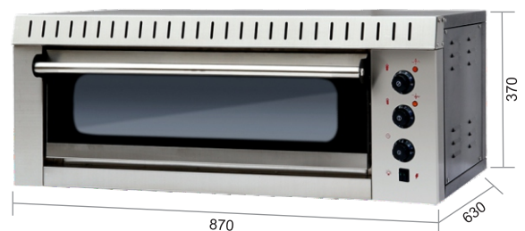
Stone Pizza Oven Big Single Deck (Full SS) Stone Size : 425x625x15mm | Power : 3Kw
